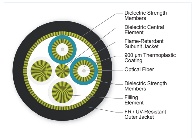
Cross Section of Part Number: 002T6F-31380-B1
