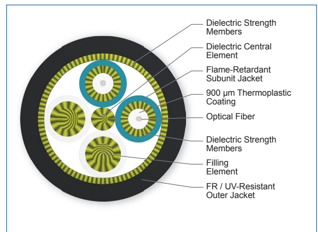
Cross Section of Part Number: 002T6F-31390-B1
