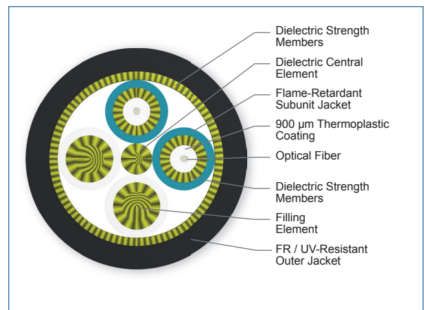
Cross Section of Part Number: 002T6F-31391-B2
