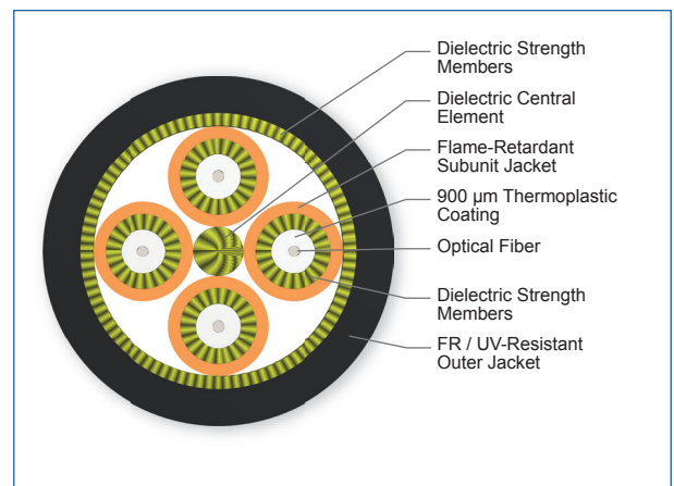
Cross Section of Part Number: 004T6F-31331-B2
