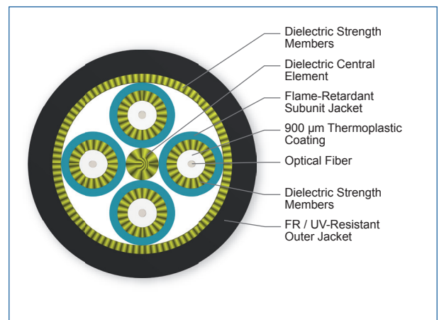
Cross Section of Part Number: 004T6F-31390-B2
