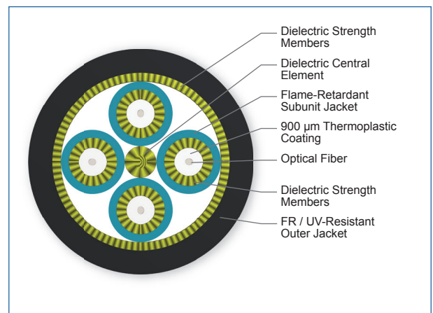
Cross Section of Part Number: 004T6F-31391-B1
