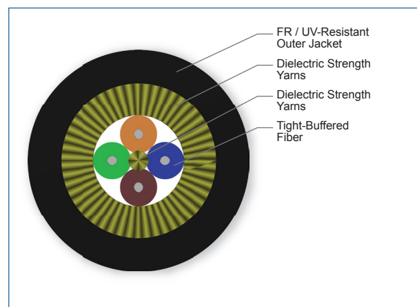
Cross Section of Part Number: 004T8F-31190-29
