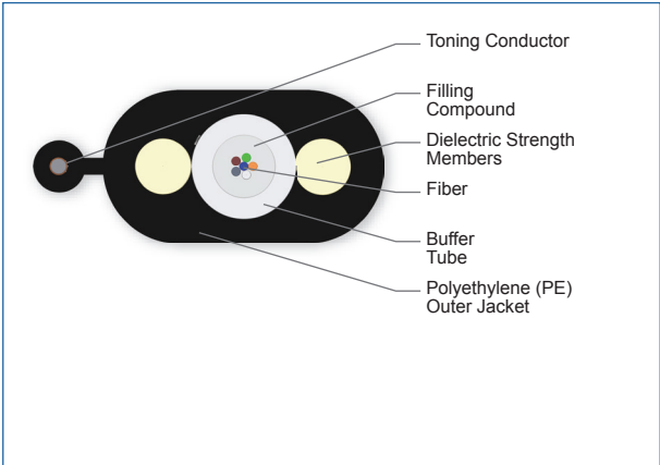
Cross Section of Part Number: 006EB1-14101A20
