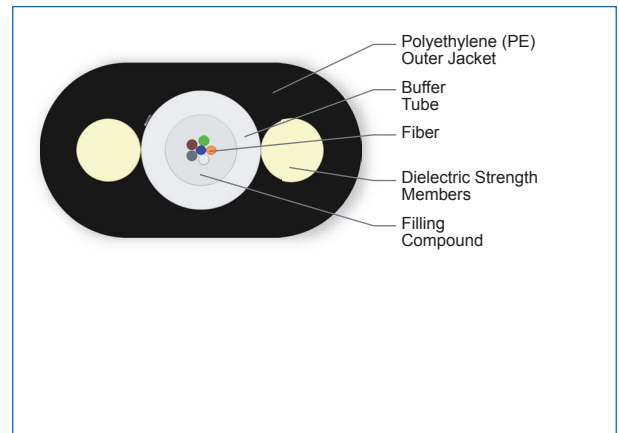
Cross Section of Part Number: 006EBZ-14101A20
