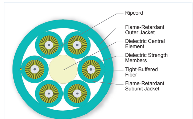
Cross Section of Part Number: 006T68-31190-29
