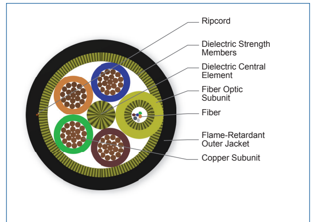
Cross Section of Part Number: 006UDF-41G01M20
