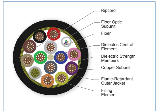
Cross Section of Part Number: 006ZTF-M1H01M20
