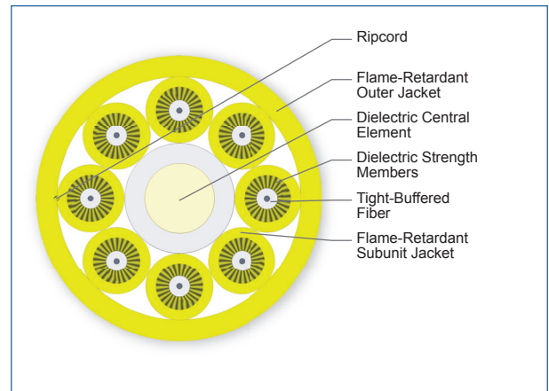
Cross Section of Part Number: 008E68-31131-29
