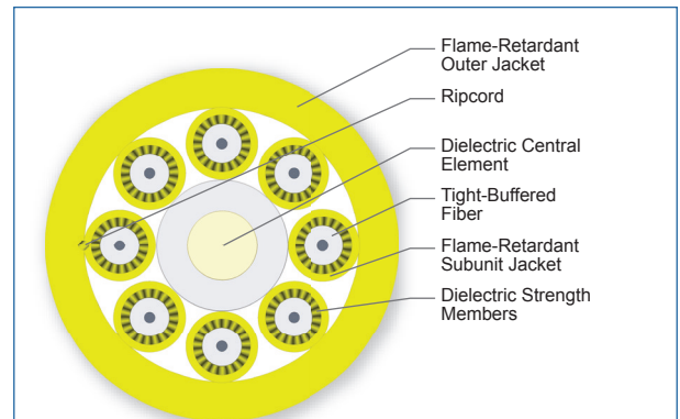
Cross Section of Part Number: 008E68-31431-29
