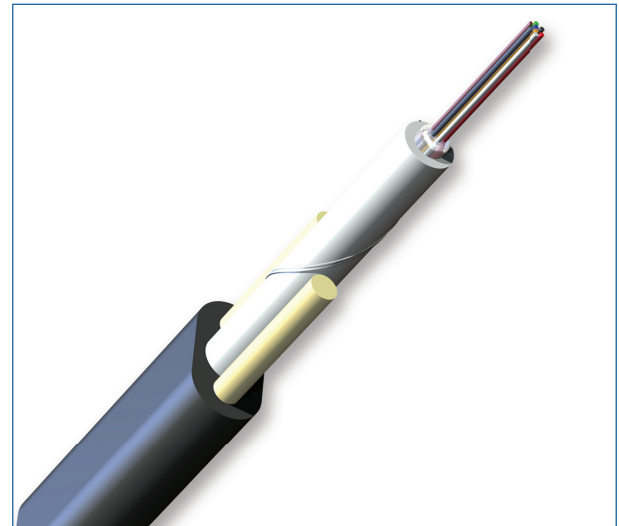
Part Number: 008EBZ-14101A20
