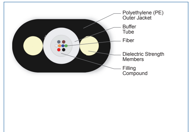
Cross Section of Part Number: 008EBZ-14101A20
