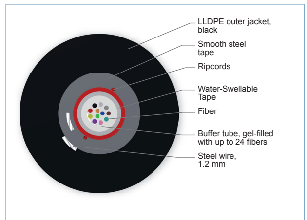
Cross Section of Part Number: 008EEW-13122A20
