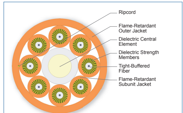
Cross Section of Part Number: 008T68-31131-29
