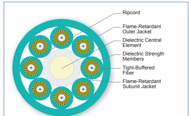
Cross Section of Part Number: 008T68-31180-29
