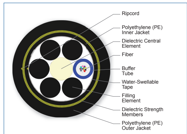
Cross Section of Part Number: 012EAE-T4201A20
