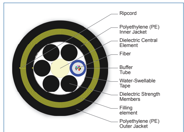
Cross Section of Part Number: 012EAE-T4A01A20
