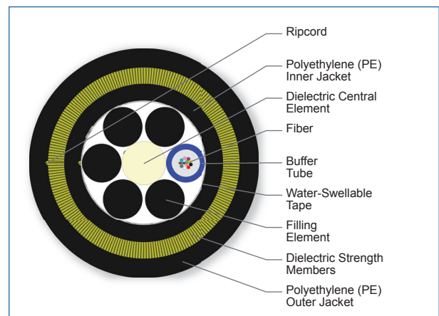
Cross Section of Part Number: 012EAE-T4C01A20
