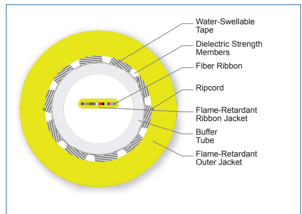
Cross Section of Part Number: 012EC8-94101-20
