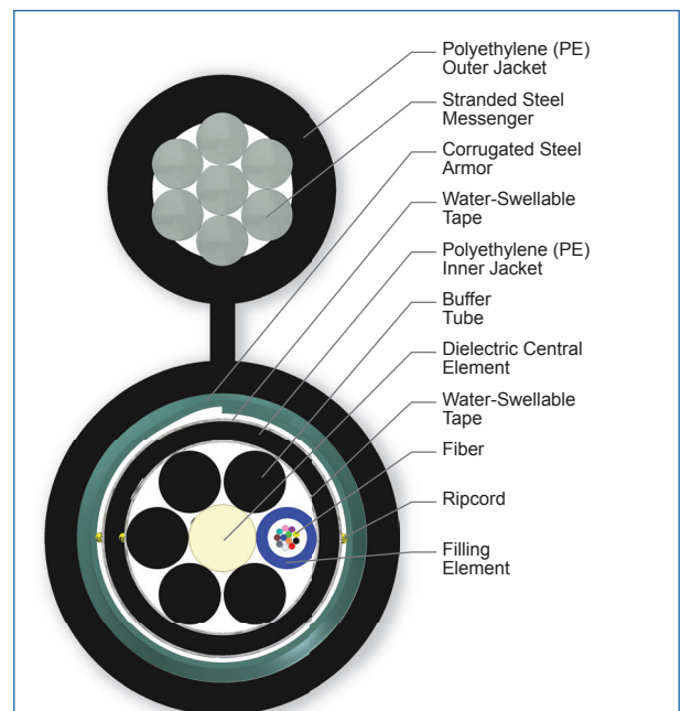
Cross Section of Part Number: 012EUB-T4101D20
