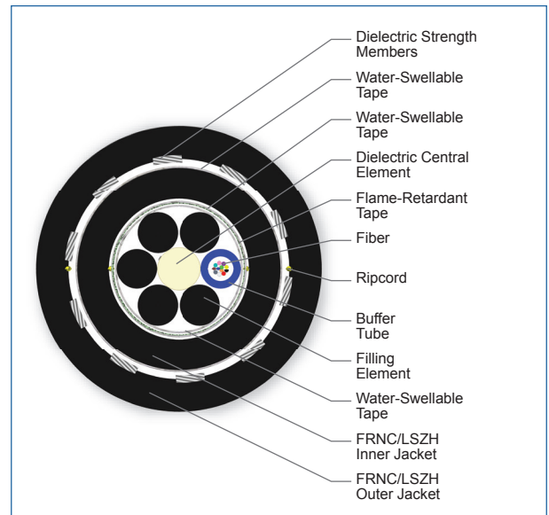
Cross Section of Part Number: 012EUL-T3601D2M
