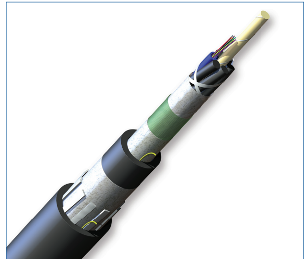
Part Number: 012EUL-T3601D2M
