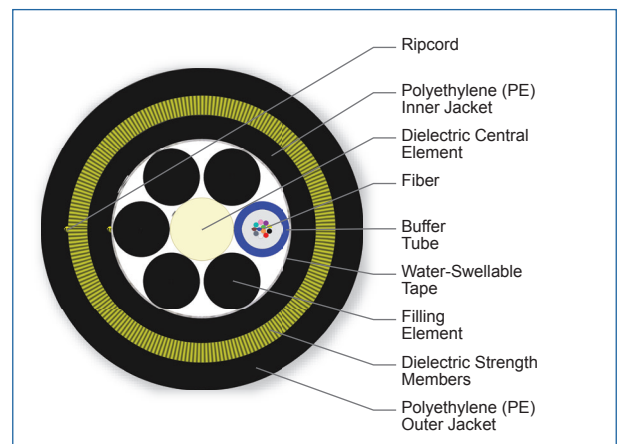
Cross Section of Part Number: 012KAE-T4A30A20
