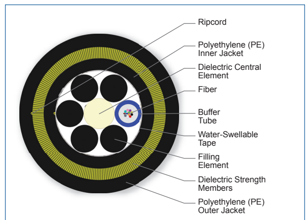
Cross Section of Part Number: 012KAE-T4C30A20
