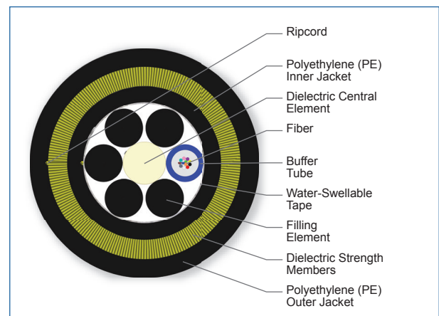
Cross Section of Part Number: 012KAE-T4E30A20
