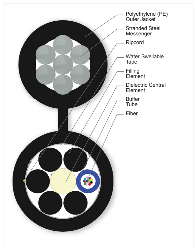
Cross Section of Part Number: 012KUA-T4130D20
