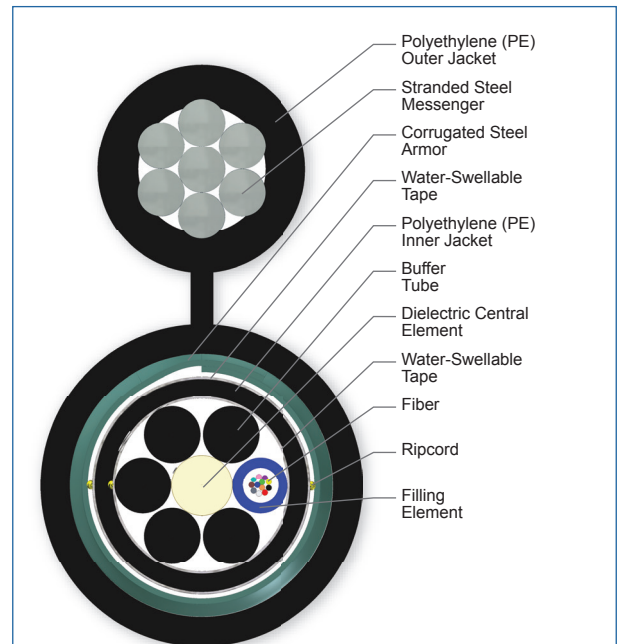
Cross Section of Part Number: 012KUB-T4130D20
