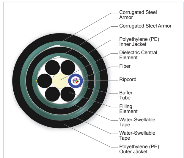
Cross Section of Part Number: 012KUD-T4130D20
