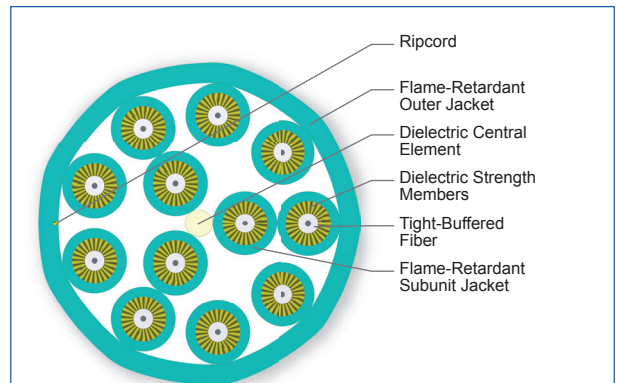
Cross Section of Part Number: 012T68-31191-29
