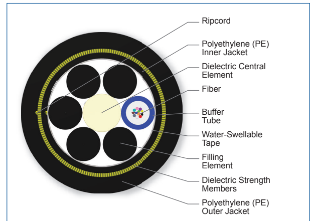
Cross Section of Part Number: 012TAE-T4231A20
