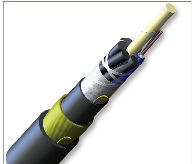
Part Number: 012TAE-T4531A20
