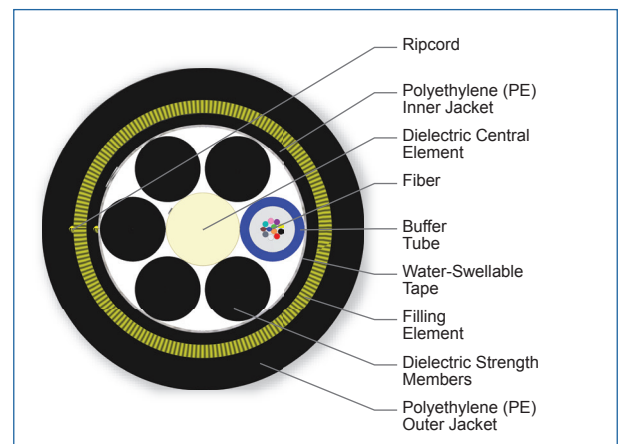
Cross Section of Part Number: 012TAE-T4531A20
