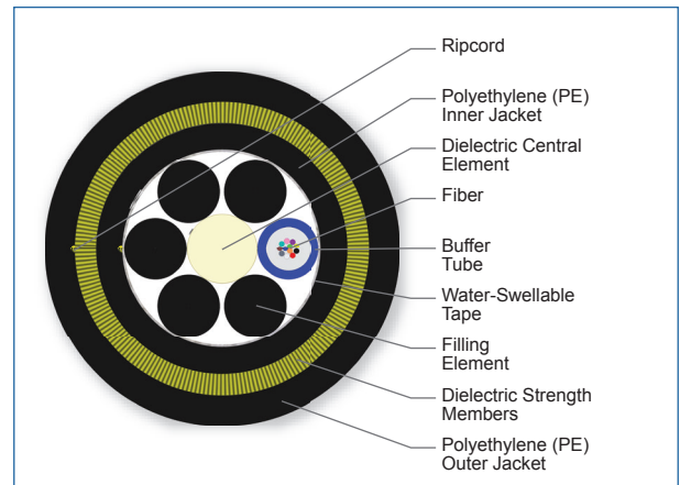
Cross Section of Part Number: 012TAE-T4A31A20
