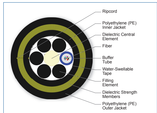
Cross Section of Part Number: 012TAE-T4C31A20
