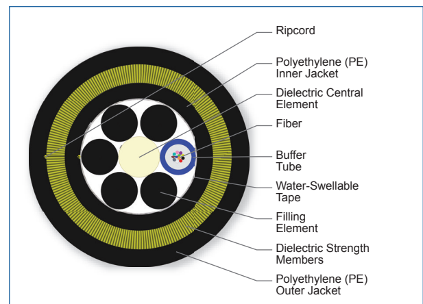
Cross Section of Part Number: 012TAE-T4E31A20
