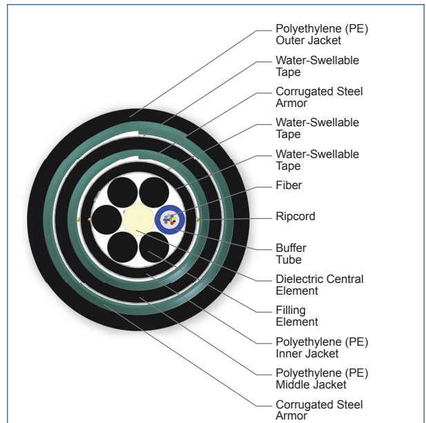
Cross Section of Part Number: 012TU6-T4131A20
