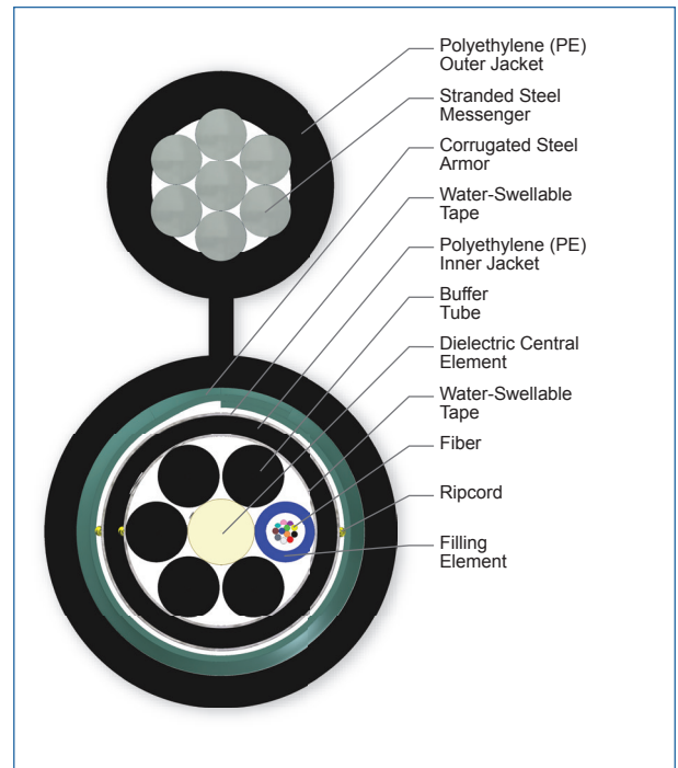
Cross Section of Part Number: 012TUB-T4131D20
