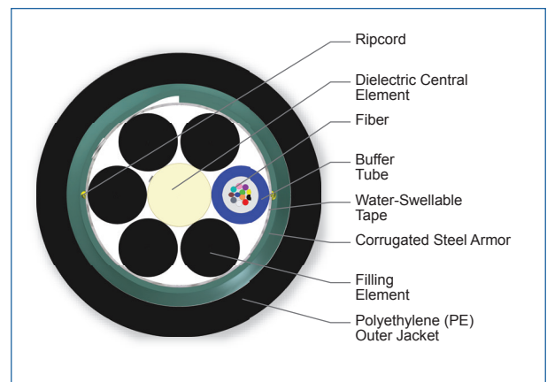
Cross Section of Part Number: 012TUC-T4131C20
