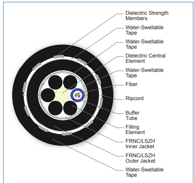
Cross Section of Part Number: 012TUL-T4690D2N
