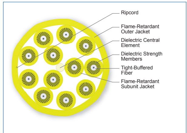
Cross Section of Part Number: 012U61-31431-24
