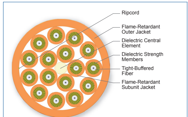
Cross Section of Part Number: 016K68-31130-29
