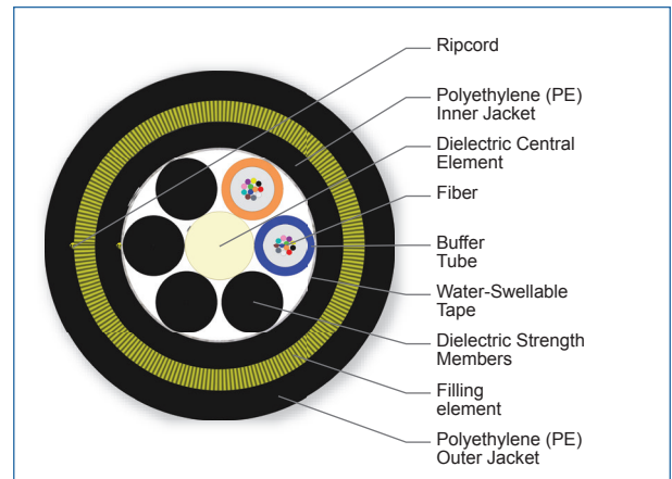
Cross Section of Part Number: 024EAE-T4A01A20
