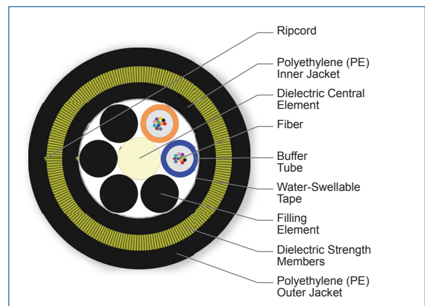
Cross Section of Part Number: 024EAE-T4C01A20
