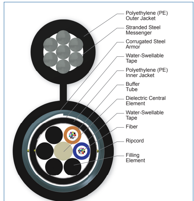
Cross Section of Part Number: 024EUB-T4101D20
