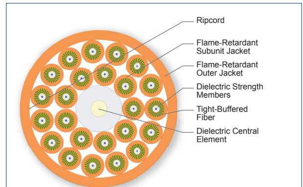
Cross Section of Part Number: 024K68-31130-29
