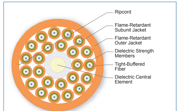
Cross Section of Part Number: 024K68-31330-29
