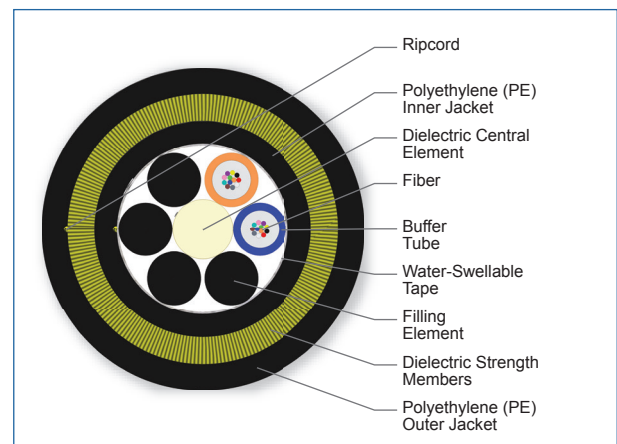
Cross Section of Part Number: 024KAE-T4E30A20
