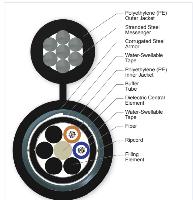
Cross Section of Part Number: 024KUB-T4130D20
