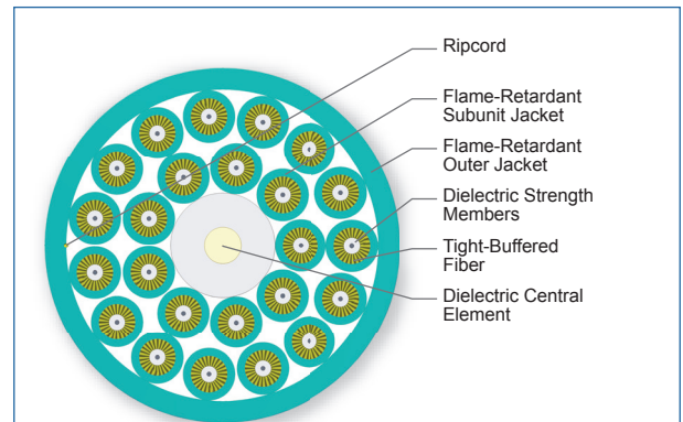
Cross Section of Part Number: 024T68-31190-29
